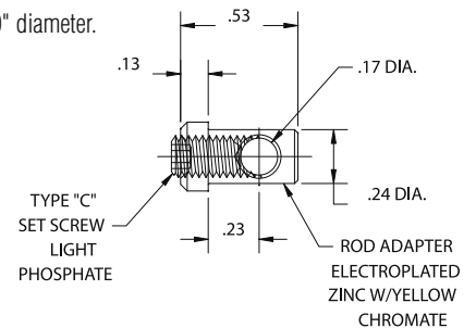
No. 1-16619-15PK Rod adapter
